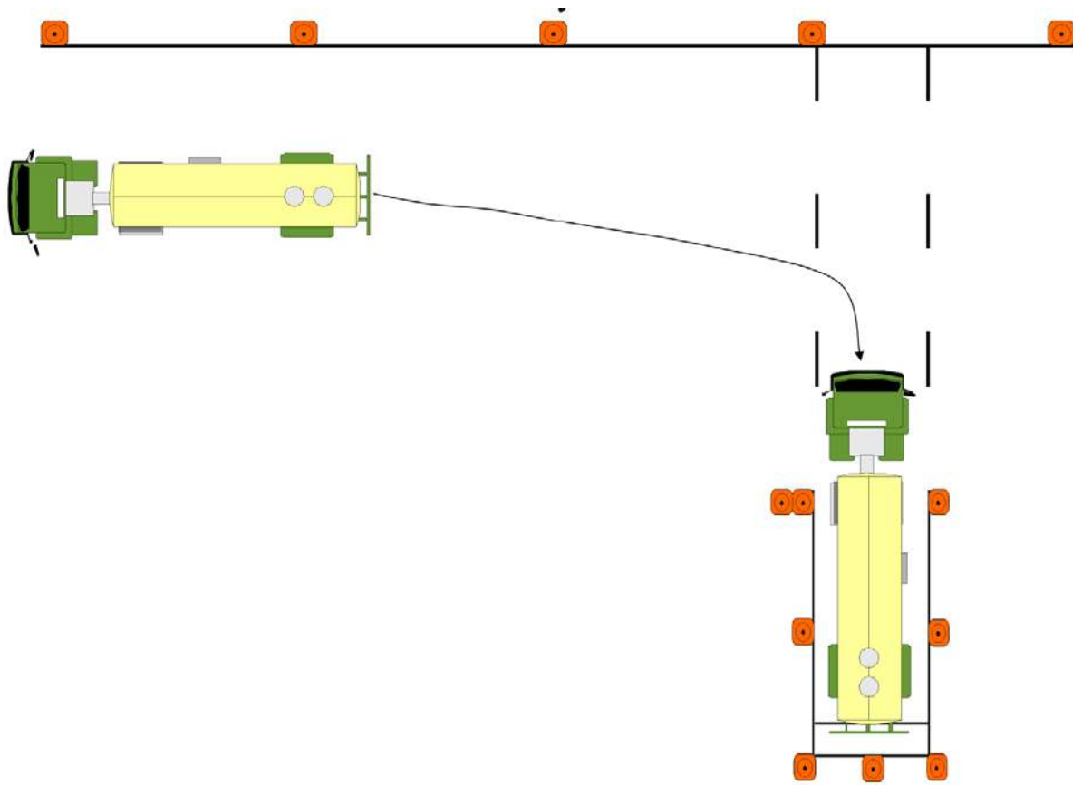
Figure 11.4: Alley Dock
